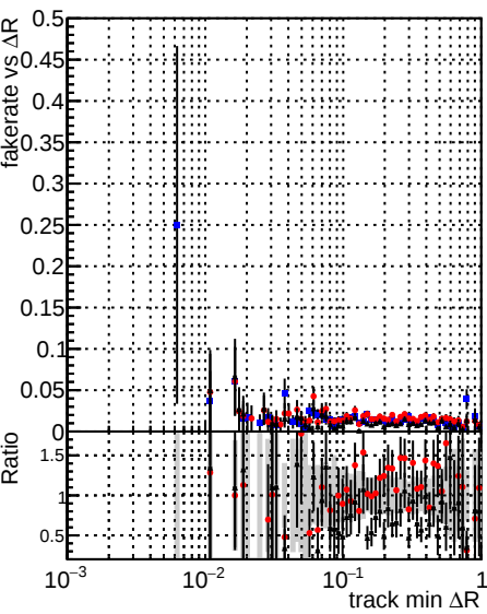
Fake rate vs ΔR(track, jet) Legend: DQM_XiMinus_original (black line with blue dots) DQM_XiMinus_newbranch_pLess (red line with red dots) DQM_XiMinus_newbranch_pLessMVACand (black line with black dots)
