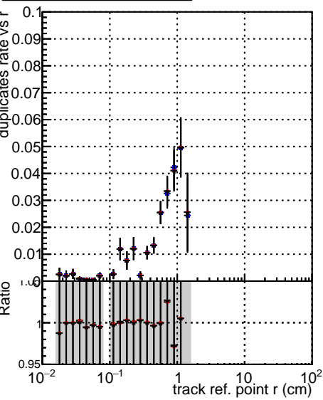
—•— DQM_XiMinus_original —•— DQM_XiMinus_newbranch_pLess —•— DQM_XiMinus_newbranch_pLessMVACand
