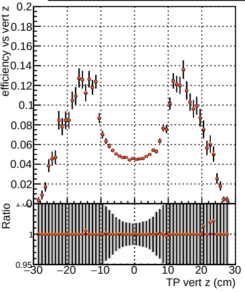
Efficiency vs vertpos DOM_XiMinus_original DOM_XiMinus_newbranch DOM_XiMinus_original_pLess DOM_XiMinus_newbranch_pLess
