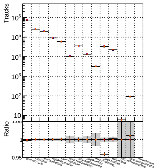
Number of tracks vs collection Legend: —●— DQM_XiMinus_original —●— DQM_XiMinus_newbranch —●— DQM_XiMinus_original_pLess —●— DQM_XiMinus_newbranch_pLess
