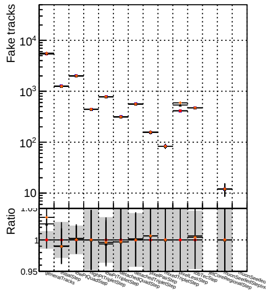
Number of tracks vs collection Legend: Blue line with circles: DQM_XiMinus_original Red line with circles: DQM_XiMinus_newbranch Black line with circles: DQM_XiMinus_original_pLess Orange line with circles: DQM_XiMinus_newbranch_pLess
