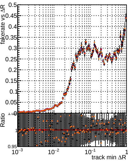
Fake rate vs \Delta R (track, jet) for different methods: DOM, XiMinus, original, newbranch, original pless, newbranch pless
