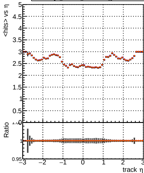
DQM_XiMinus_original DQM_XiMinus_newbranch DQM_XiMinus_original_pLess DQM_XiMinus_newbranch_pLess mean hits
