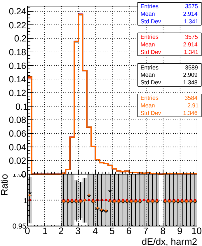
Legend for bottom row plots: DQM_XiMinus_original (Blue line with circles) DQM_XiMinus_newbranch (Red line with circles) DQM_XiMinus_original_pLess (Black line with circles) DQM_XiMinus_newbranch_pLess (Orange line with circles)
