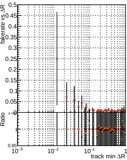
Fake rate vs \Delta R(\text{track, jet}) Legend: DOM (black), XiMinus (blue), original (red), newbranch (orange) DOM XiMinus original newbranch DOM XiMinus original newbranch DOM XiMinus original newbranch DOM XiMinus original newbranch
