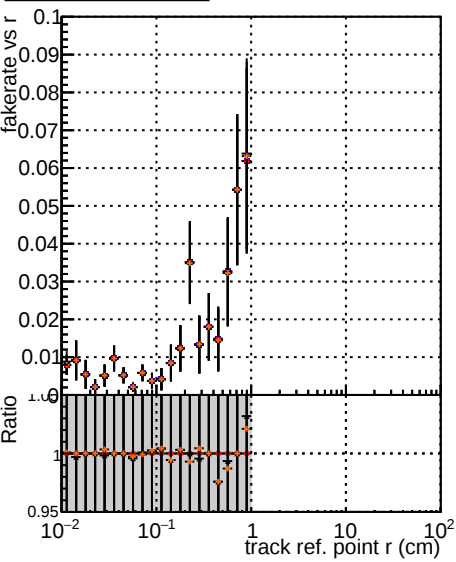
Fake rate vs v Legend: DOM X-Minus original (blue square) DOM X-Minus newbranch (red circle) DOM X-Minus original pless (black triangle) DOM X-Minus newbranch pless (orange diamond)
