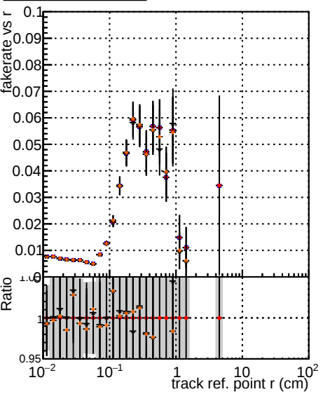
Fake rate vs verpos Legend: DOM XMinus original (blue) DOM XMinus newbranch (red) DOM XMinus original pless (black) DOM XMinus newbranch pless (orange)
