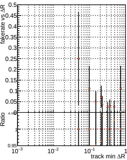
Fake rate vs ΔR(track, jet) Legend: DOM (black line) XiMinus (blue line) original (red line) newbranch (orange line)
