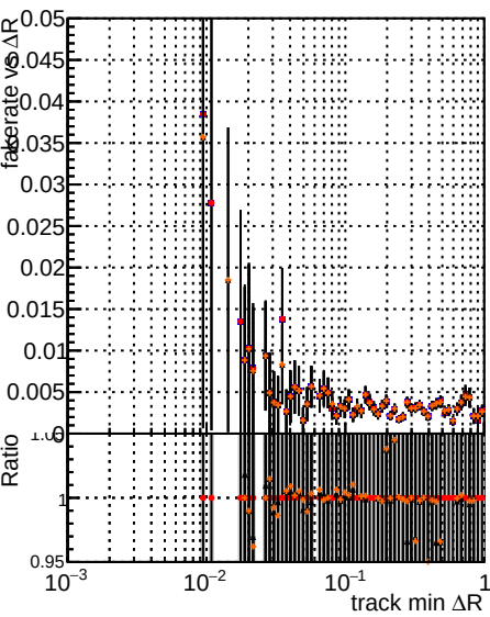
Fake rate vs \Delta R (track, jet) Legend: DOM X Minus original DOM X Minus newbranch DOM X Minus original pless DOM X Minus newbranch pless
