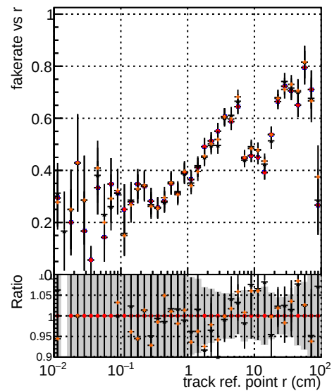
DOM X Minus original DOM X Minus newbranch DOM X Minus original pless DOM X Minus newbranch pless
