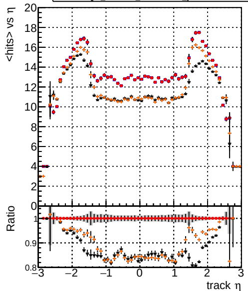
DQM_XiMinus_original DQM_XiMinus_newbranch DQM_XiMinus_original_pLess DQM_XiMinus_newbranch_pLess mean hits
