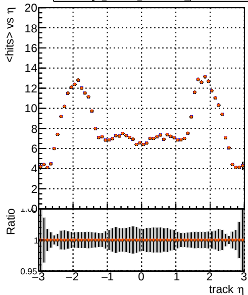
mean hits DQM_XiMinus_original DQM_XiMinus_newbranch DQM_XiMinus_original_pLess DQM_XiMinus_newbranch_pLess
