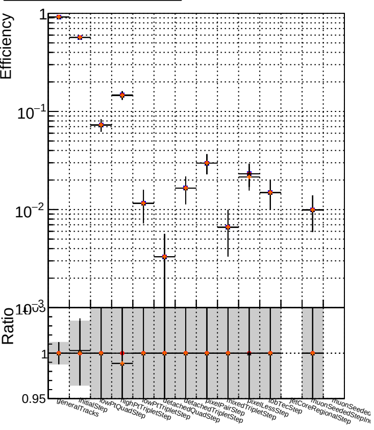
DQM_XiMinus_original DQM_XiMinus_newbranch DQM_XiMinus_original_pLess DQM_XiMinus_newbranch_pLess
