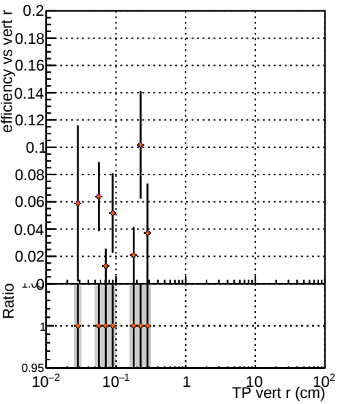
Efficiency vs vertpos — DQM_XiMinus_original — DQM_XiMinus_newbranch — DQM_XiMinus_original_pLess — DQM_XiMinus_newbranch_pLess
