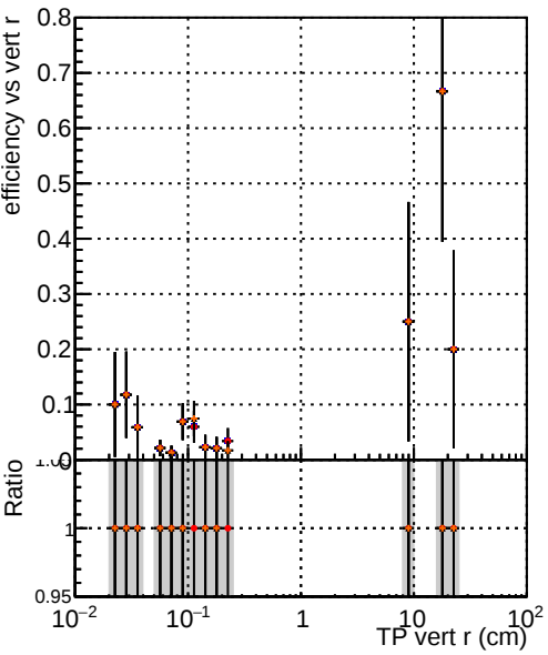
Efficiency vs TP vert r (cm) —•— DQM_XiMinus_original —•— DQM_XiMinus_newbranch —•— DQM_XiMinus_original_pLess —•— DQM_XiMinus_newbranch_pLess
