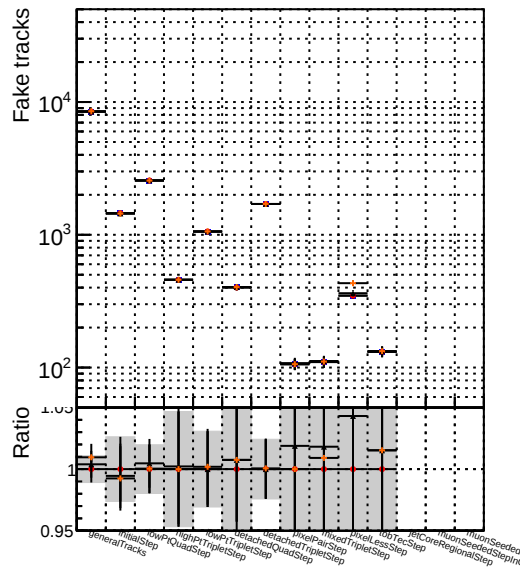
Number of tracks vs collection Legend: QOM_XiMinus_original QOM_XiMinus_newbranch QOM_XiMinus_original_pLess QOM_XiMinus_newbranch_pLess
