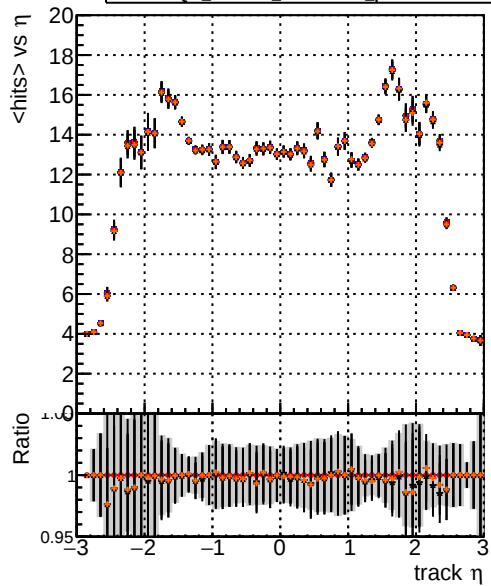
Legend: DQM_XiMinus_original (blue line), DQM_XiMinus_newbranch (red line with dots), DQM_XiMinus_original_pLess (black line with dots), DQM_XiMinus_newbranch_pLess (orange line with dots) mean hits
