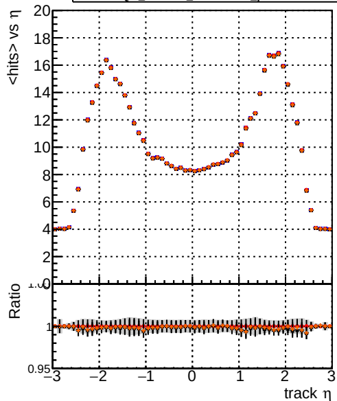
DQM_XiMinus_original DQM_XiMinus_newbranch DQM_XiMinus_original_pLess DQM_XiMinus_newbranch_pLess
