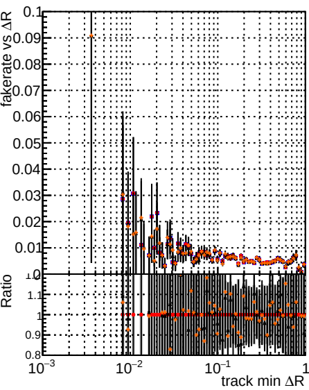
Fake rate vs \Delta R (track, jet) for different methods: DOM, X-Minus, original, newbranch, original pless, newbranch pless
