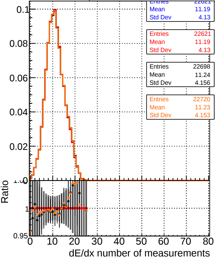
—●— DQM_XiMinus_original —●— DQM_XiMinus_newbranch —●— DQM_XiMinus_original_pLess —●— DQM_XiMinus_newbranch_pLess
