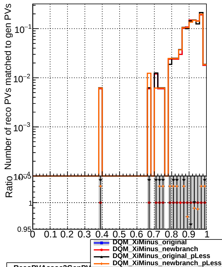
RecoPVAssoc2GenPVMatched_missing
