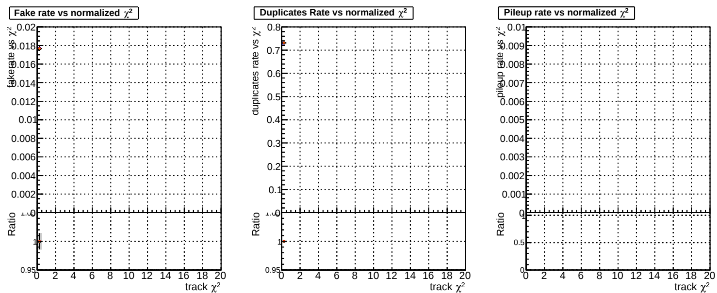
Fake rate vs. \chi^2
