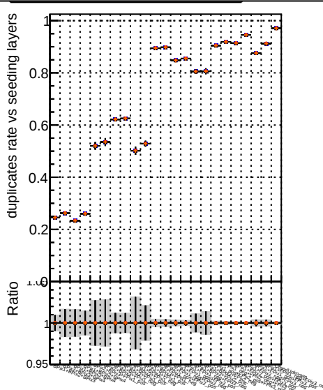
Duplicates Rate vs \chi^2
