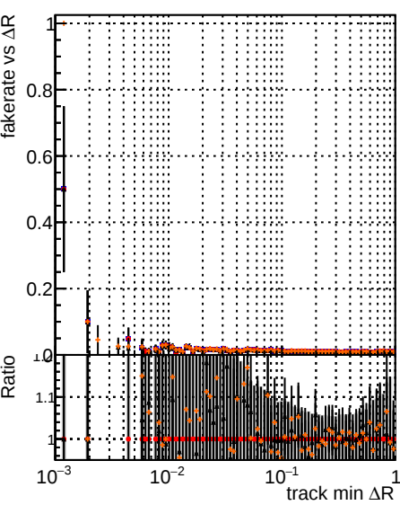
Fake rate vs \Delta R(\text{track, jet}) DOM X minus original DOM X minus newbranch DOM X minus original pless DOM X minus newbranch pless
