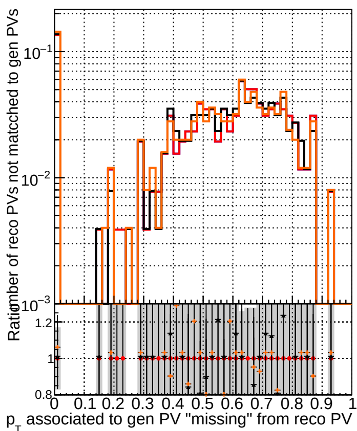
RecoPVAssoc2GenPVnotmatched_missing
