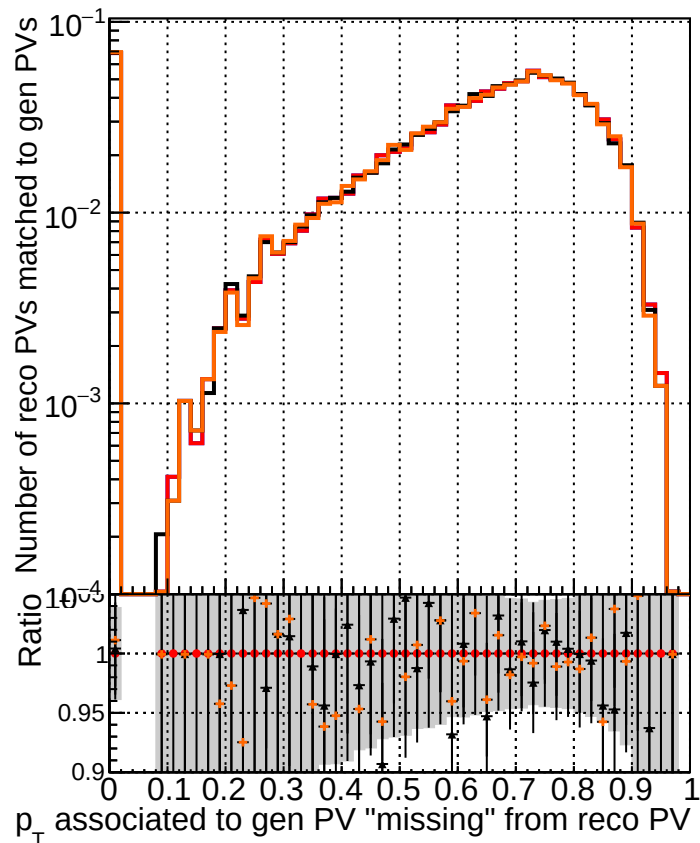
RecoPVAssoc2GenPVmatched_missing
