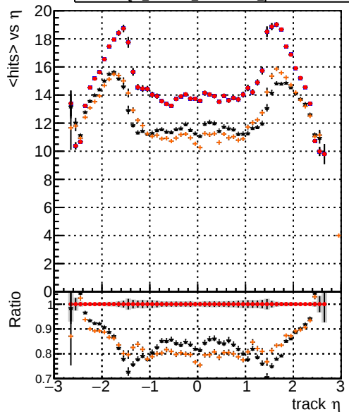
Legend: — DQM_XiMinus_original — DQM_XiMinus_newbranch — DQM_XiMinus_original_pLess — DQM_XiMinus_newbranch_pLess mean hits
