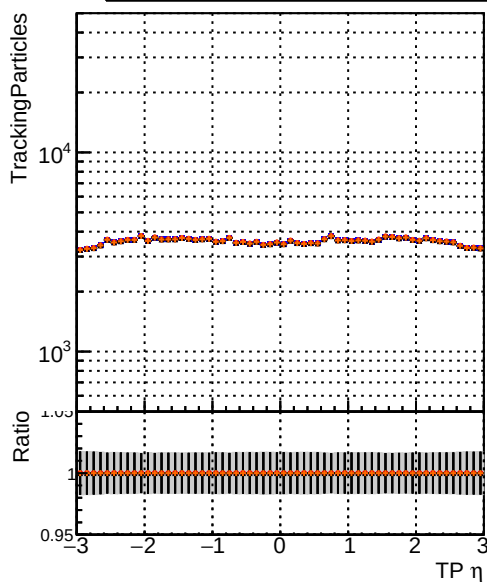
Legend: - DQM_XiMinus_original (blue line with circles) - DQM_XiMinus_newbranch (red line with diamonds) - DQM_XiMinus_original_pLess (black line with triangles) - DQM_XiMinus_newbranch_pLess (orange line with squares)
