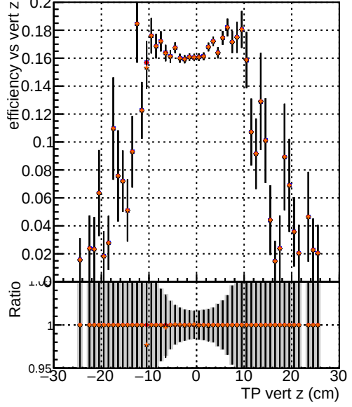
Efficiency vs. TP vert z (cm) —•— DQM_XiMinus_original —•— DQM_XiMinus_newbranch —•— DQM_XiMinus_original_pLess —•— DQM_XiMinus_newbranch_pLess
