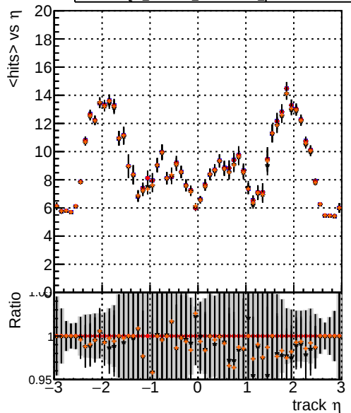
DQM_XiMinus_original DQM_XiMinus_newbranch DQM_XiMinus_original_pLess DQM_XiMinus_newbranch_pLess
