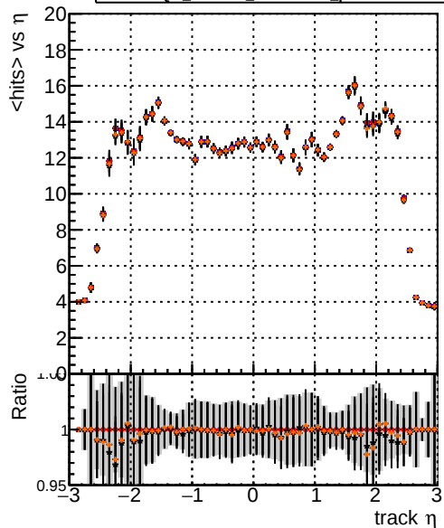
Legend: DQM_XiMinus_original (blue line), DQM_XiMinus_newbranch (red line), DQM_XiMinus_original_pLess (black line), DQM_XiMinus_newbranch_pLess (orange line) mean hits
