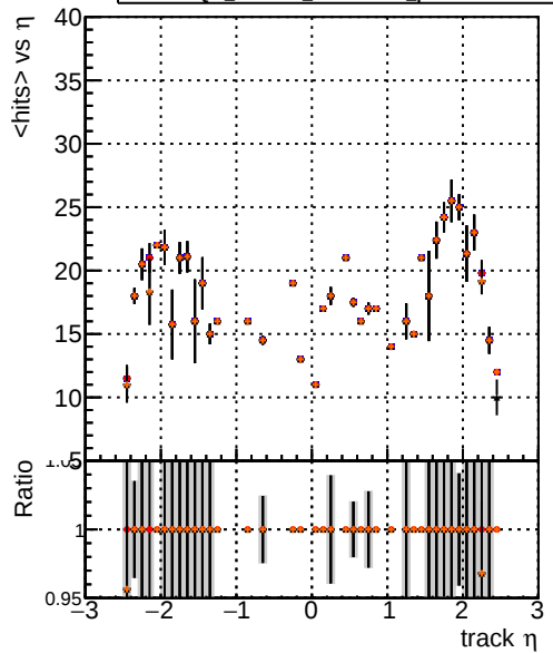
Legend: — DQM_XiMinus_original — DQM_XiMinus_newbranch — DQM_XiMinus_original_pLess — DQM_XiMinus_newbranch_pLess
