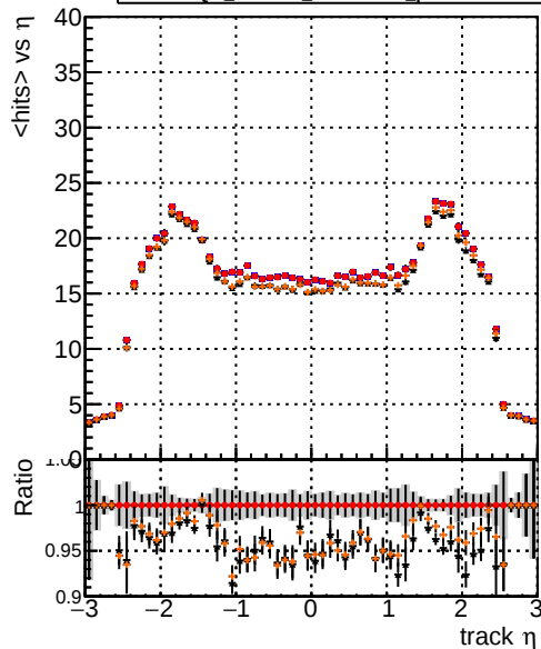
mean hits vs \eta Legend: DQM_XiMinus_original (blue line), DQM_XiMinus_newbranch (red line), DQM_XiMinus_original_pLess (black line with error bars), DQM_XiMinus_newbranch_pLess (orange line with error bars)
