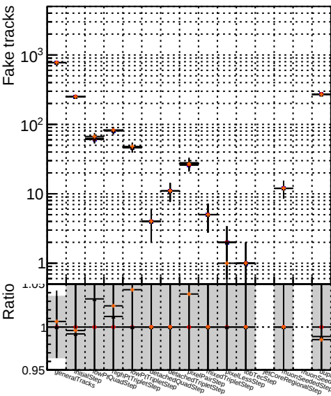
Number Legend 1 DQM_XiMinus_original_pLess 2 DQM_XiMinus_newbranch_pLess
