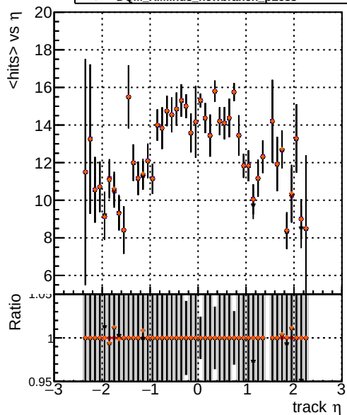
DQM_XiMinus_original DQM_XiMinus_newbranch DQM_XiMinus_original_pLess DQM_XiMinus_newbranch_pLess mean hits
