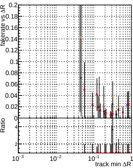
Fake rate vs ΔR(track, jet) for different models and pT thresholds
