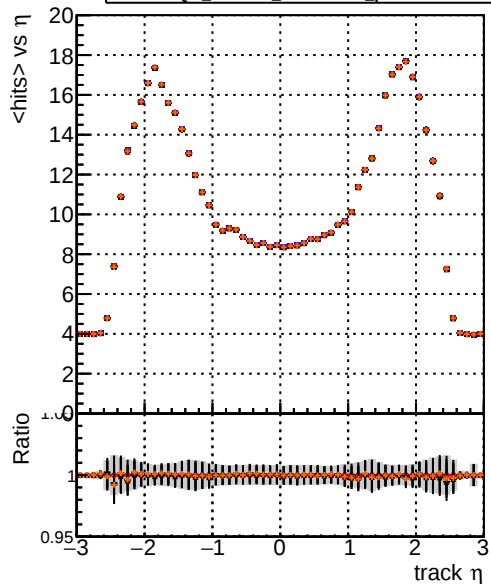
mean hit DQM_XiMinus_original DQM_XiMinus_newbranch DQM_XiMinus_original_pLess DQM_XiMinus_newbranch_pLess
