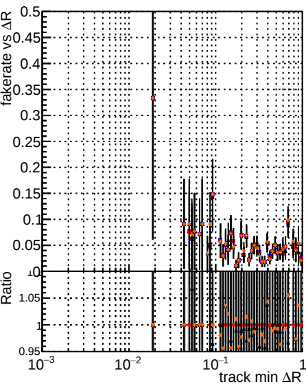
Fake rate vs \Delta R(\text{track}, \text{jet}) Legend: original (black), newbranch (red), original plus (blue)
