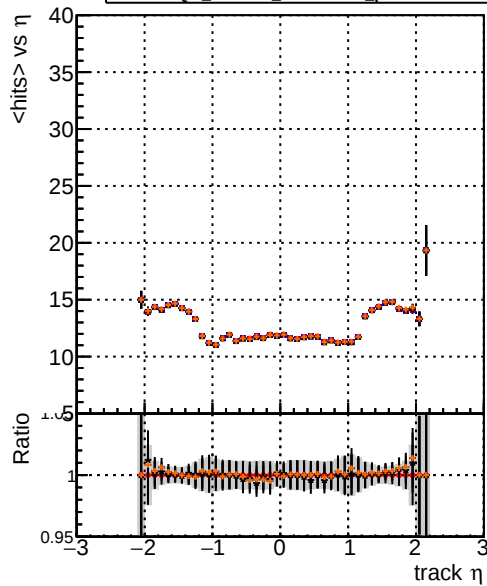
Legend: - DQM_XiMinus_original (blue line) - DQM_XiMinus_newbranch (red line) - DQM_XiMinus_original_pLess (grey line) - DQM_XiMinus_newbranch_pLess (orange line)
