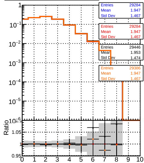
Legend: - DQM_XiMinus_original (blue line) - DQM_XiMinus_newbranch (red line) - DQM_XiMinus_original_pLess (grey line) - DQM_XiMinus_newbranch_pLess (orange line)
