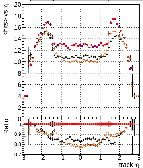
mean hits vs \eta Legend: DQM_XiMinus_original (blue line), DQM_XiMinus_newbranch (red line), DQM_XiMinus_original_pLess (black line), DQM_XiMinus_newbranch_pLess (orange line)
