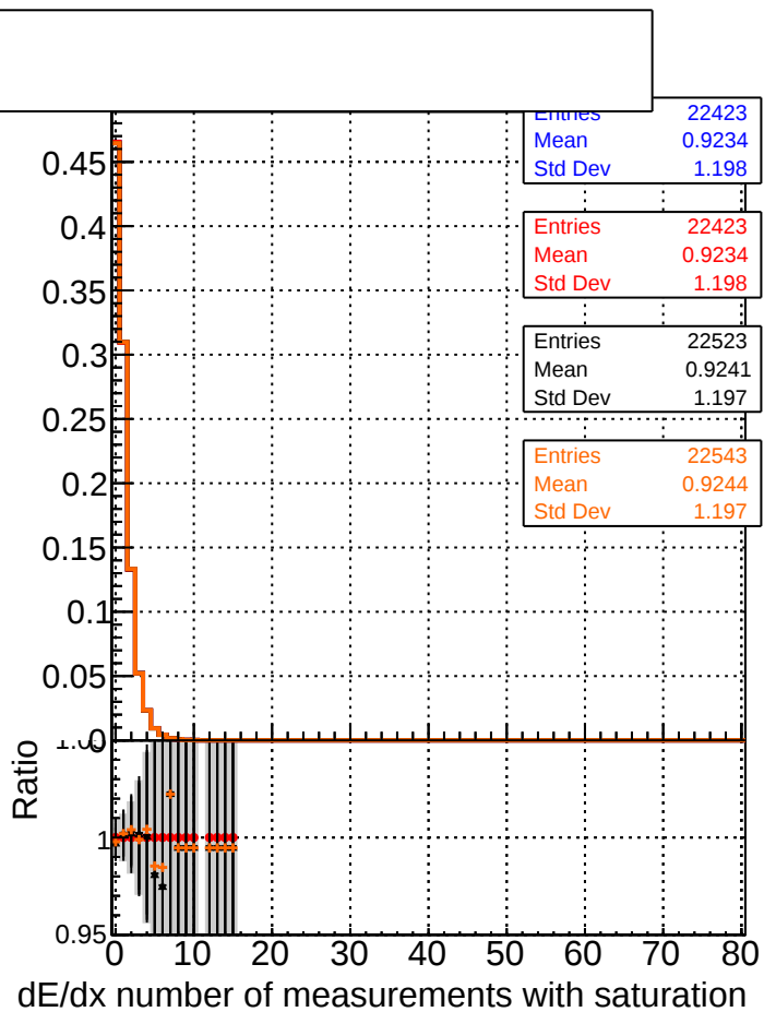
—●— DQM_XiMinus_original —●— DQM_XiMinus_newbranch —●— DQM_XiMinus_original_pLess —●— DQM_XiMinus_newbranch_pLess
