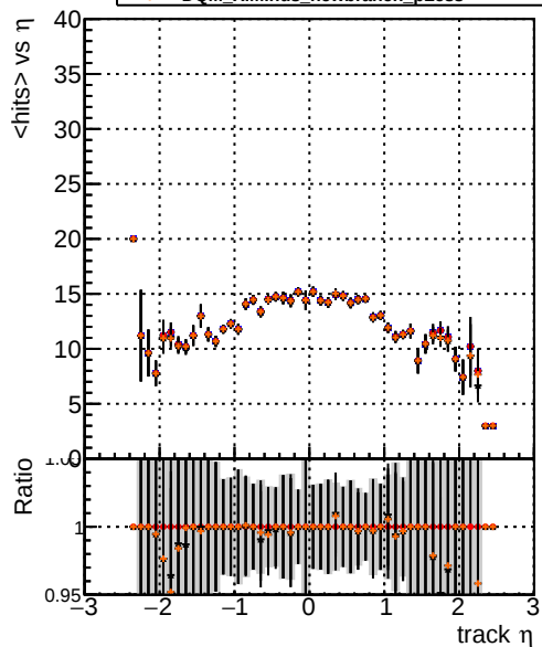
mean hits vs \eta DQM_XiMinus_original DQM_XiMinus_newbranch DQM_XiMinus_original_pLess DQM_XiMinus_newbranch_pLess
