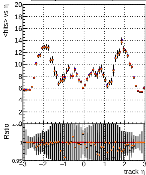
mean hit Legend: Blue line: DQM_XiMinus_original Red line: DQM_XiMinus_newbranch Black line: DQM_XiMinus_original_pLess Orange line: DQM_XiMinus_newbranch_pLess
