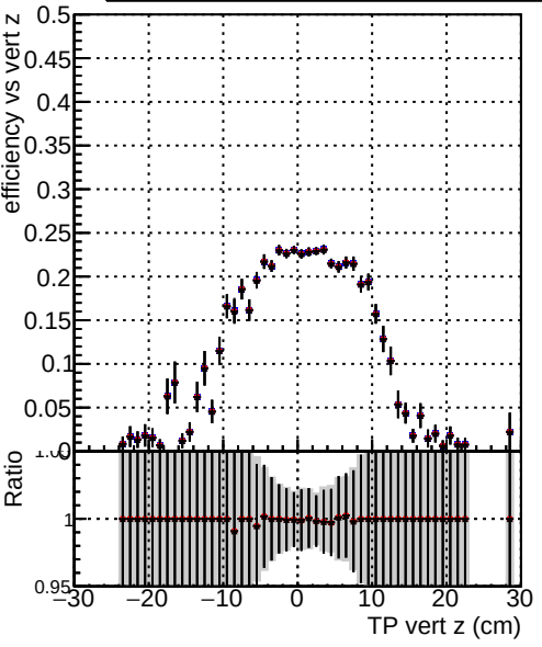
Efficiency vs vertpos DQM_TT_original_lowpt DQM_TT_newbranch_lowpt_pLess DQM_TT_newbranch_lowpt_pLessMVACand
