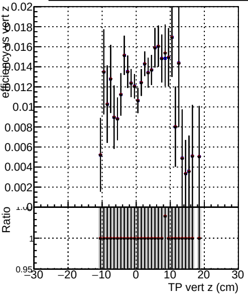
Efficiency vs TP vert z (cm) Legend: DQM_TT_original_lowpt (Blue line with circles) DQM_TT_newbranch_lowpt_pLess (Red line with circles) DQM_TT_newbranch_lowpt_pLessMVACand (Black line with circles)
