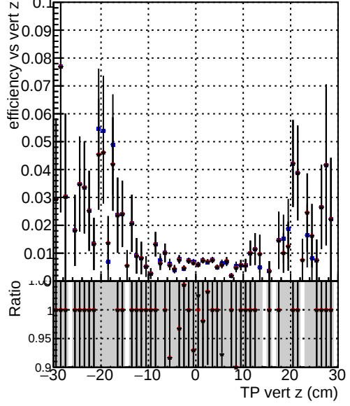
Efficiency vs. TP vert z —•— DQM_TT_original_lowpt —•— DQM_TT_newbranch_lowpt_pLess —•— DQM_TT_newbranch_lowpt_pLessMVACand
