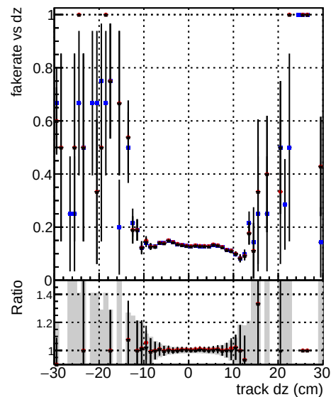
Fake rate vs dz Legend: DOM TT original lowpt, DOM TT newbranch lowpt pLess, DOM TT newbranch lowpt pLessMVACand
