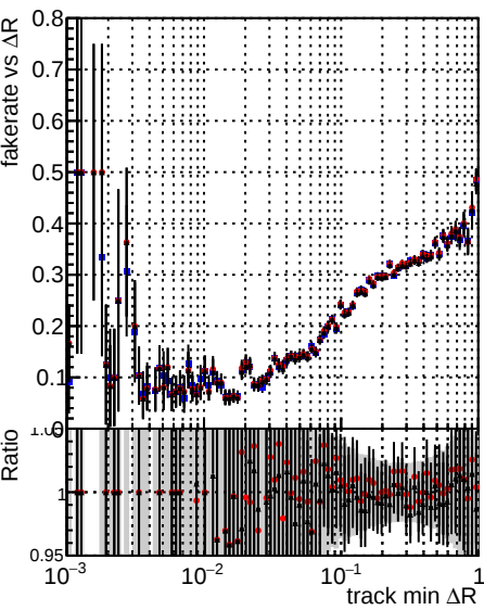
Fake rate vs \Delta R(\text{track, jet}) Legend: DQM TT original_lowpt (blue circles) DQM TT newbranch_lowpt_pLess (red circles) DQM TT newbranch_lowpt_pLessMVACand (black circles)
